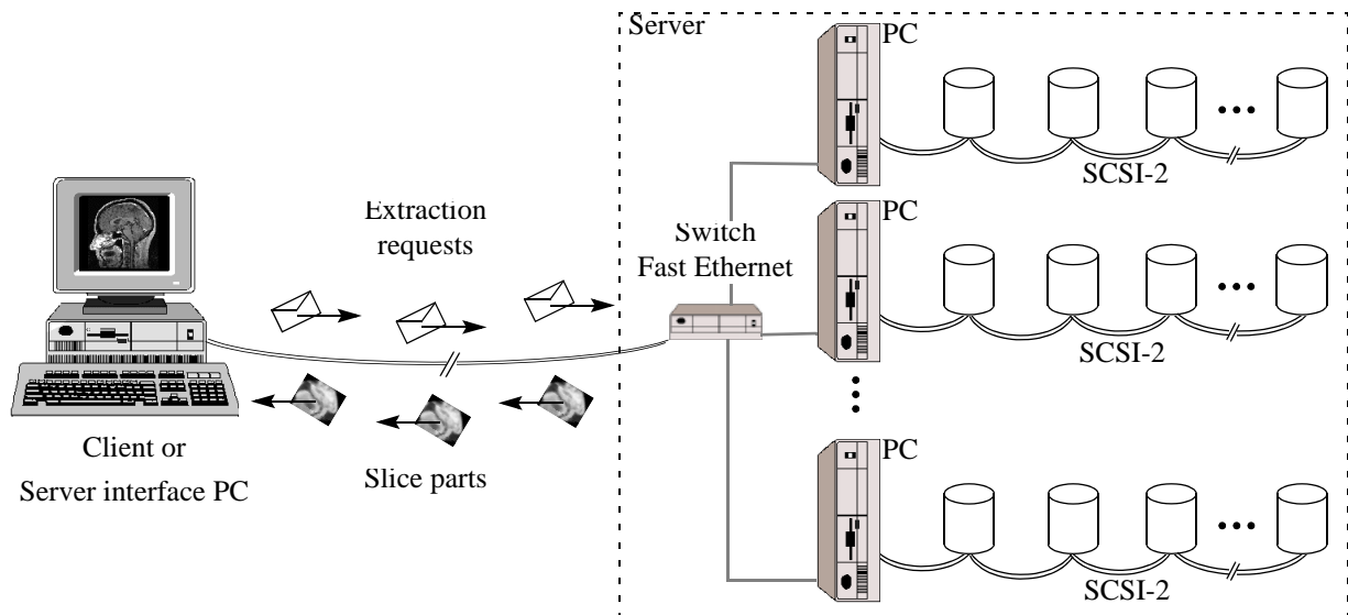
Fig. 3 Sending the slice extraction requests and receiving slice parts.
