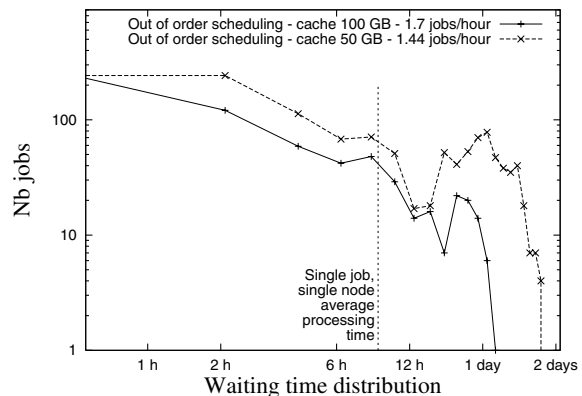
Figure 4: Waiting time distribution for the out of order scheduling policy near the maximal sustainable load.
