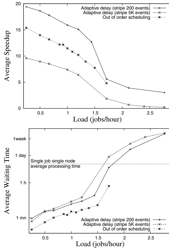
Figure 7: Speedup and waiting time (delay included) of the adaptive delay policy for different stripe sizes (cache 100 GB) compared with the out of order scheduling policy
