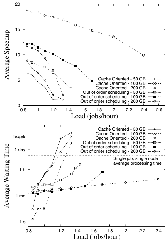
Figure 3: Average speedup and waiting time for cache-oriented job splitting and out of order scheduling policies
