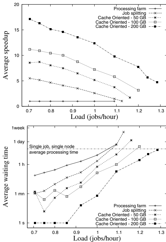
Figure 2: Average speedup and waiting time for different scheduling policies, different cache sizes and different load levels for a system comprising 10 processing nodes
