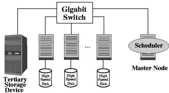
Figure 1: Architecture of the simulated cluster
