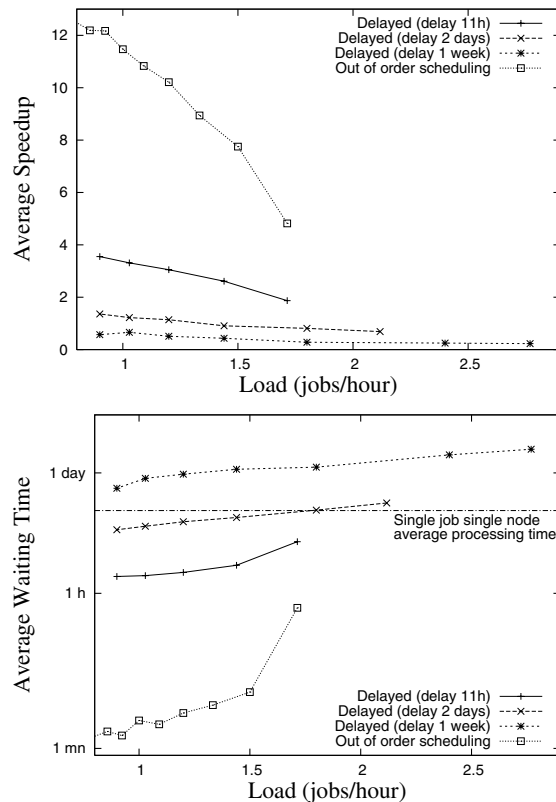
Figure 5: Speedup and waiting time (delay excluded) of the delayed scheduling policy for different delays (cache size 100 GB, stripe size 5000 events)
