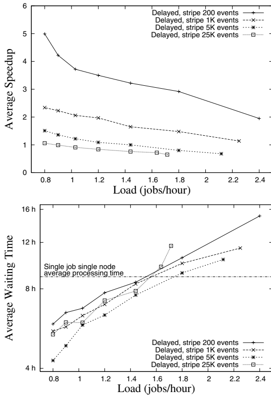
Figure 6: Average speedup and waiting time (delay excluded) of delayed scheduling for different stripe sizes (cache size 100 GB, period delay 2 days)
