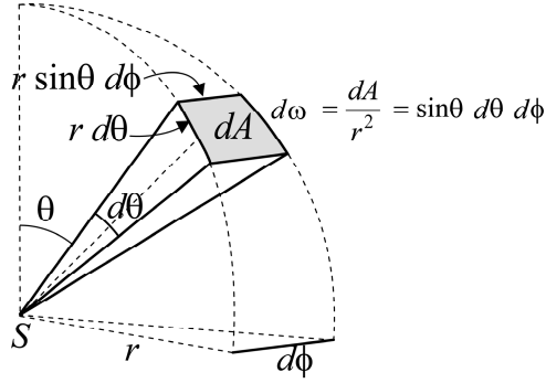
Figure 11. Infinitesimal solid angle d\omega = \sin\theta d\theta d\phi
