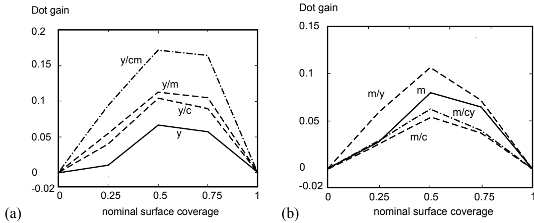
Figure 15: Dot gain as a function of nominal surface coverage, for ink halftones printed alone (solid line) and in superposition with the other solid inks (dotted lines), in the case of (a) an offset print at 150 lpi and (b) a thermal transfer print at 75 lpi.
