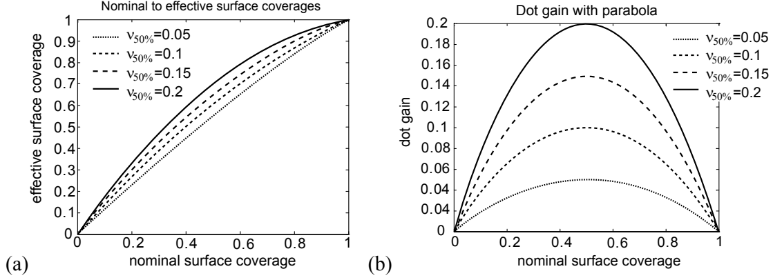
Figure 14: (a) Nominal to effective surface coverages given by the parabola Eq. (71) and (b) corresponding dot gain curve expressed by the parabola Eq. (72).
