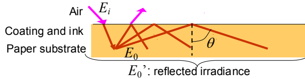
Figure 10. Irradiance elements reflected by the paper bulk.
