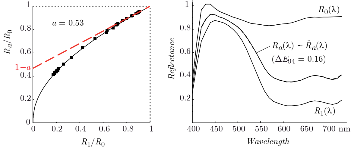
Figure 22: Comparison of predicted and measured spectral reflectances of cyan ink printed at 0.5 nominal surface coverage. Left: diagram representing the curve predicted according to equation (85) (black solid curve) and the measured points (R_1/R_0, R_a/R_0) at the different wavelengths. The red dashed line represents the reflectance that would be obtained if the halftone would behave as predicted by the simple Spectral Neugebauer model. Right: measured spectral reflectances of the unprinted paper R_0(\lambda) , of the halftone R_a(\lambda) and of the solid ink patch R_1(\lambda) as well as predicted reflectance \hat{R}_a(\lambda) of the halftone.
