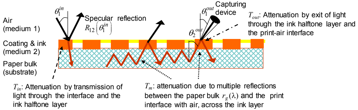
Figure 12: Path of a collimated beam of light from the source to the detector, with multiple internal reflections between the substrate and the colored layer-air interface.
