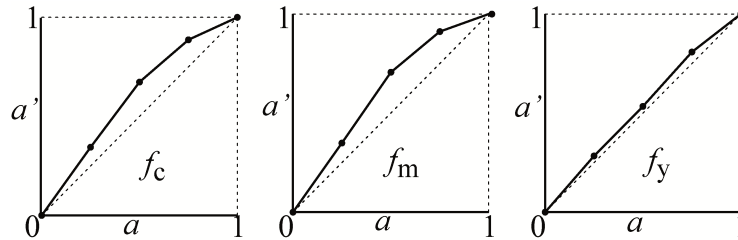
Figure 19. Example of ink spreading curves f_i obtained by linear interpolation of the effective surface coverages a_i' which are deduced from measurement of patches with single-ink halftones (ink i ) printed at nominal surface coverages 0.25, 0.5 and 0.75 (IIS method).
