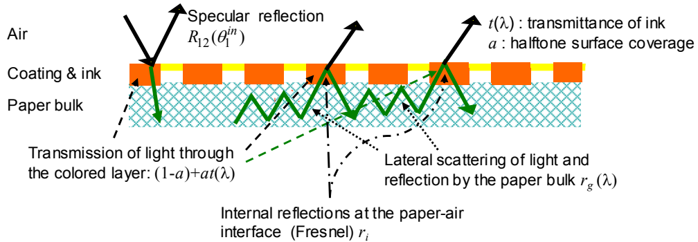
Figure 9: Phenomena accounted for by the Clapper-Yule model.
