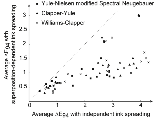
Figure 21: Comparison between the prediction accuracy offered by independent and superposition-dependent ink spreading, for three prediction models, for the sets of halftones listed in the Appendix. The smaller the \Delta E_{94} difference, the higher the prediction accuracy.
