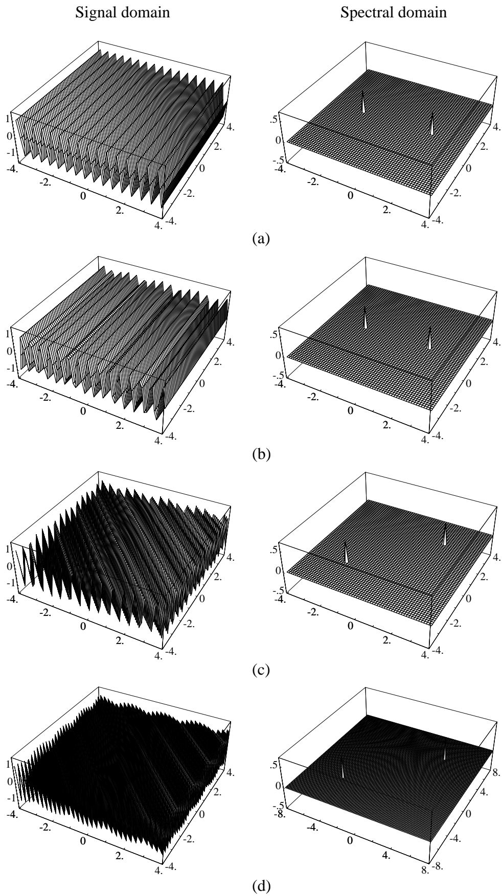
Figure subnyq2D12a from the DFT Demonstration Kit Accompanying the book: Mastering the Discrete Fourier Transform in One, Two or Several Dimensions: Pitfalls and Artifacts by I. Amidror, published by Springer, 2013.
