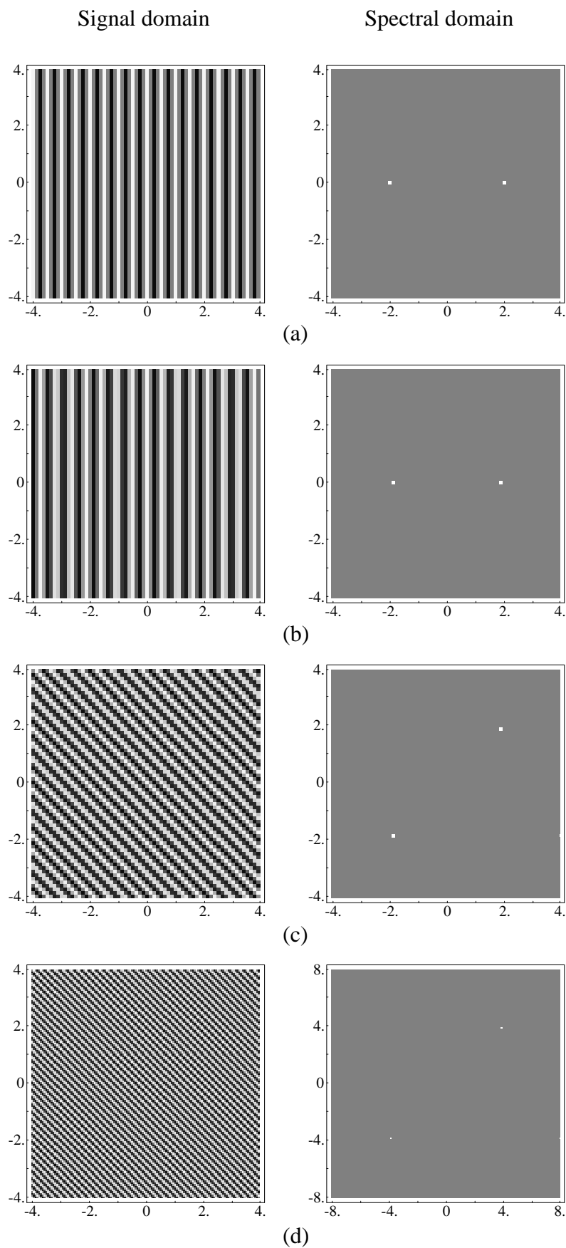
Figure subnyq2D12 from the DFT Demonstration Kit Accompanying the book: Mastering the Discrete Fourier Transform in One, Two or Several Dimensions: Pitfalls and Artifacts by I. Amidror, published by Springer, 2013.
