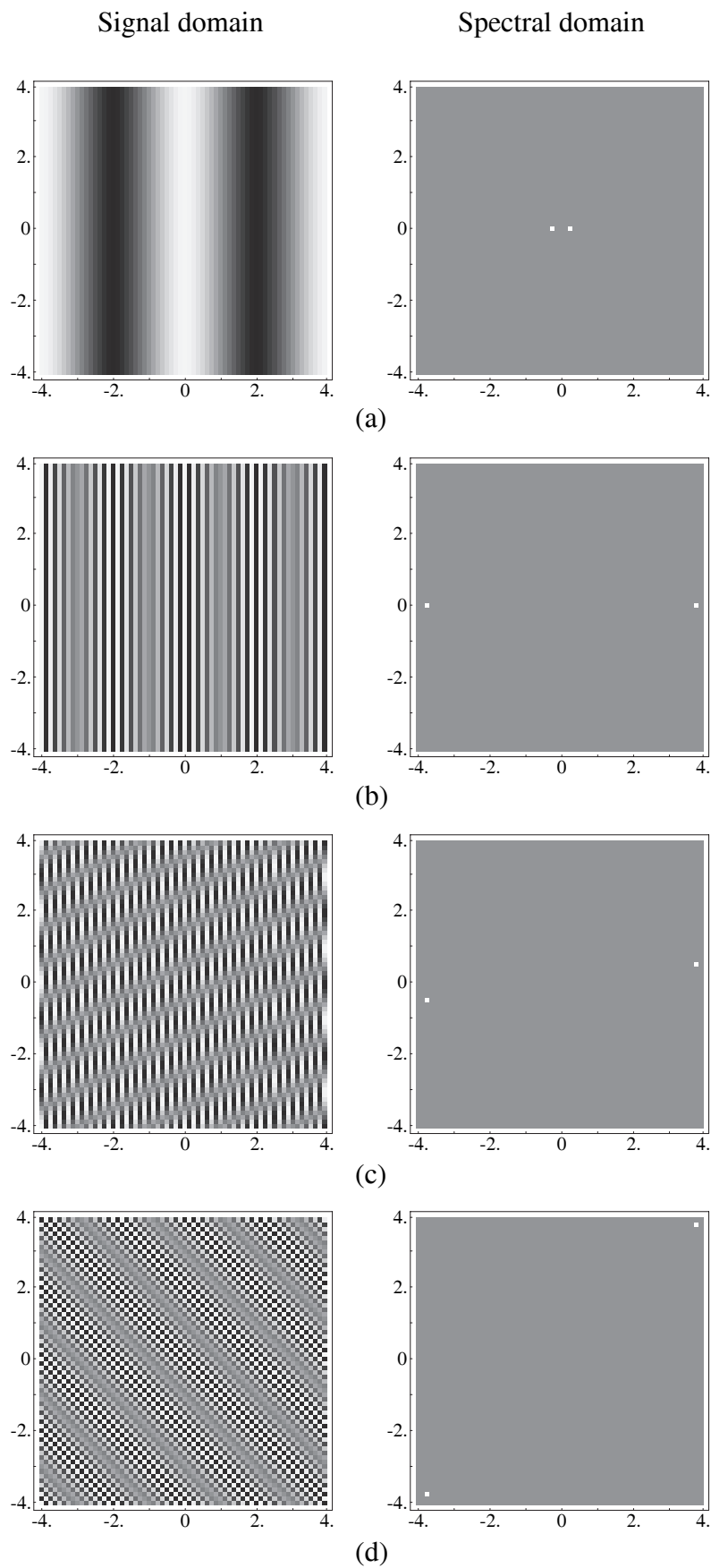
Figure subnyq2D from the DFT Demonstration Kit Accompanying the book: Mastering the Discrete Fourier Transform in One, Two or Several Dimensions: Pitfalls and Artifacts by I. Amidror, published by Springer, 2013.
