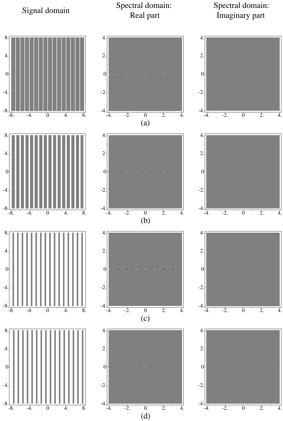
Figure grat from the DFT Demonstration Kit Accompanying the book: Mastering the Discrete Fourier Transform in One, Two or Several Dimensions: Pitfalls and Artifacts by I. Amidror, published by Springer, 2013.
