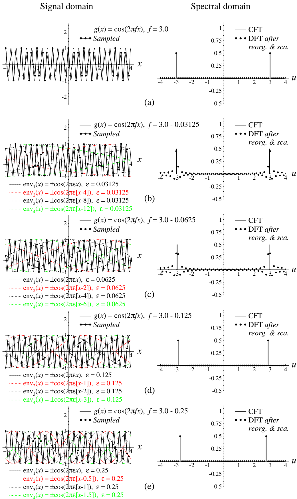
Figure cosfreq5 from the DFT Demonstration Kit Accompanying the book: Mastering the Discrete Fourier Transform in One, Two or Several Dimensions: Pitfalls and Artifacts by I. Amidror, published by Springer, 2013.
