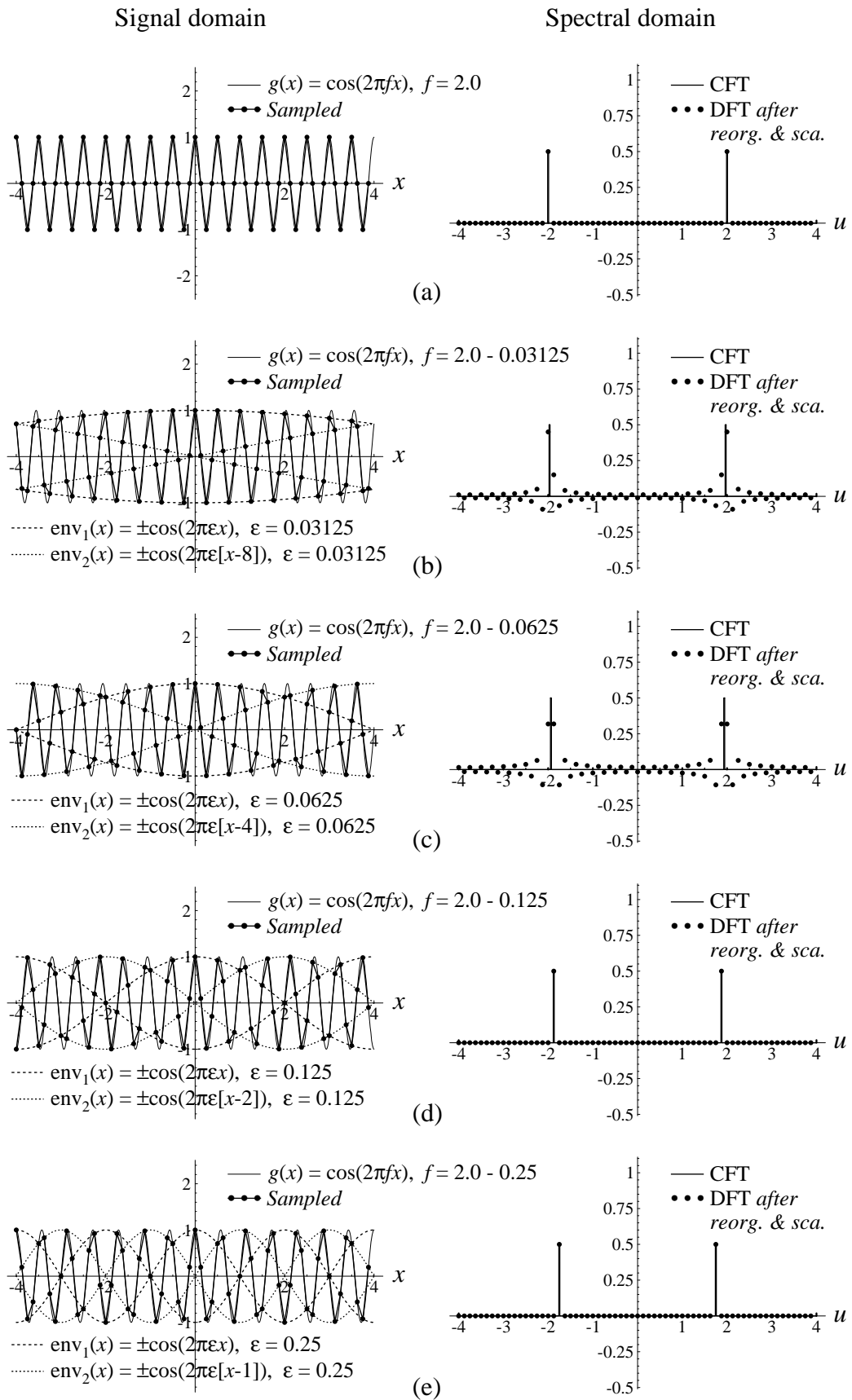
Figure cosfreq3 from the DFT Demonstration Kit Accompanying the book: Mastering the Discrete Fourier Transform in One, Two or Several Dimensions: Pitfalls and Artifacts by I. Amidror, published by Springer, 2013.
