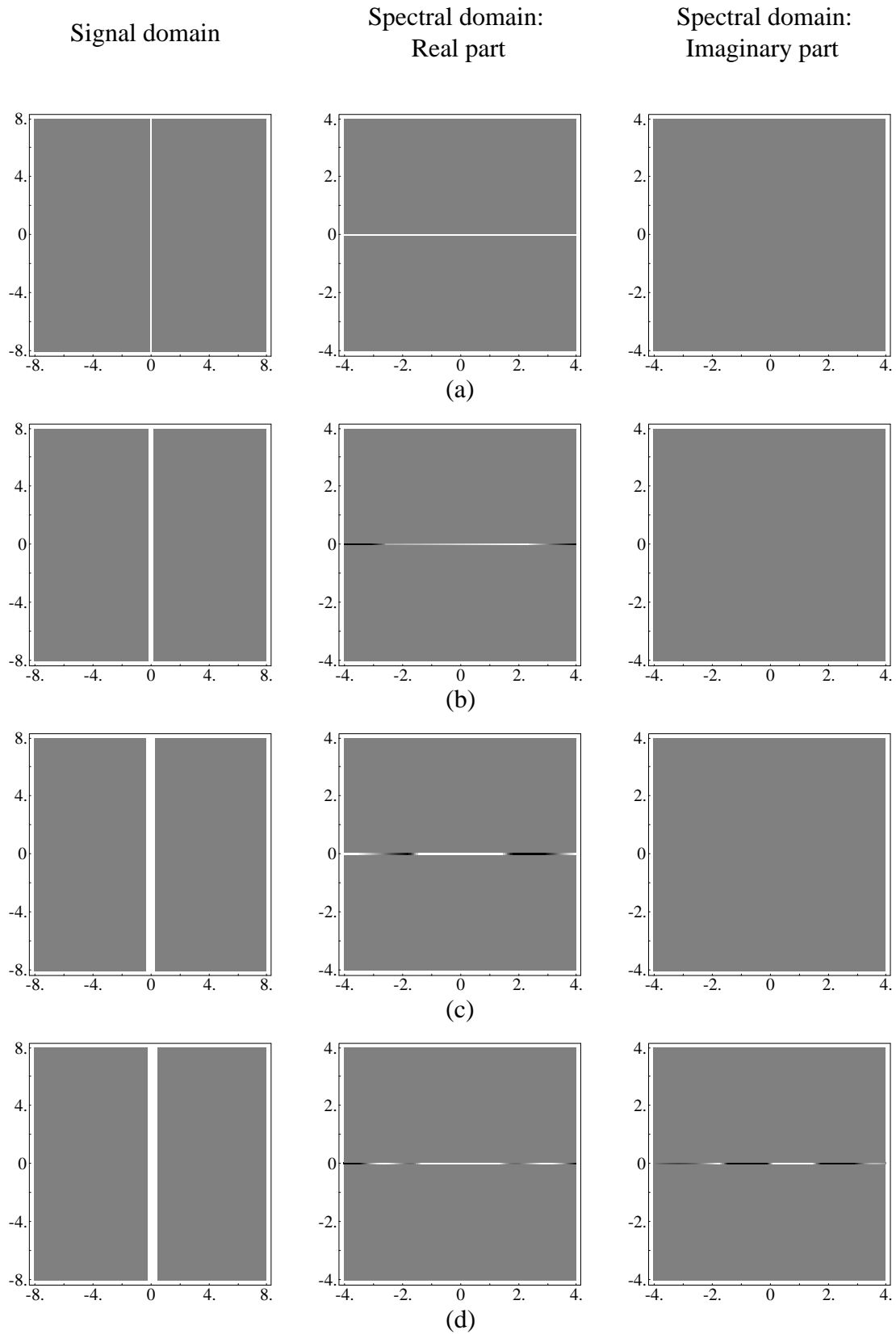
Figure bar from the DFT Demonstration Kit Accompanying the book: Mastering the Discrete Fourier Transform in One, Two or Several Dimensions: Pitfalls and Artifacts by I. Amidror, published by Springer, 2013.
